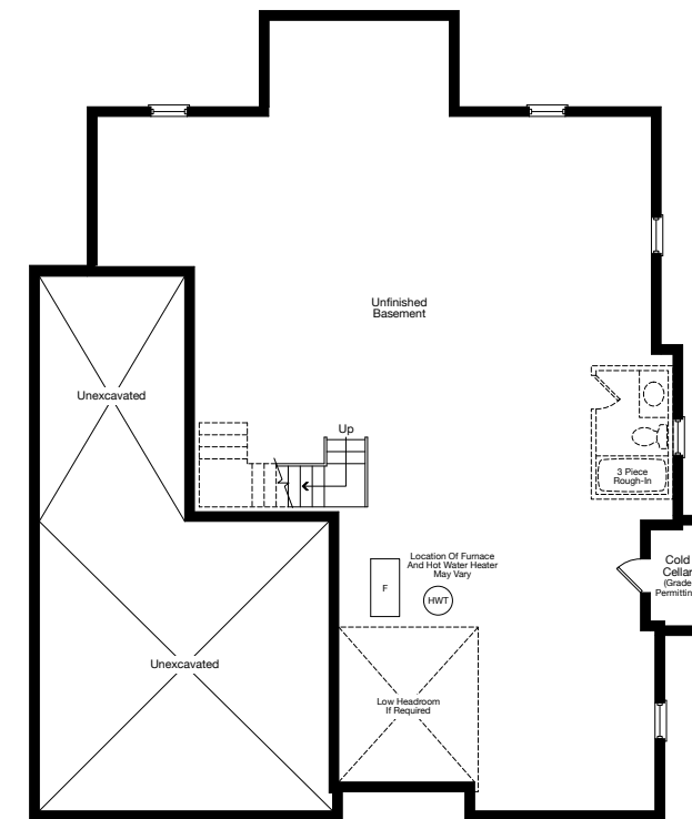
BASEMENT ELEVATION A & B
