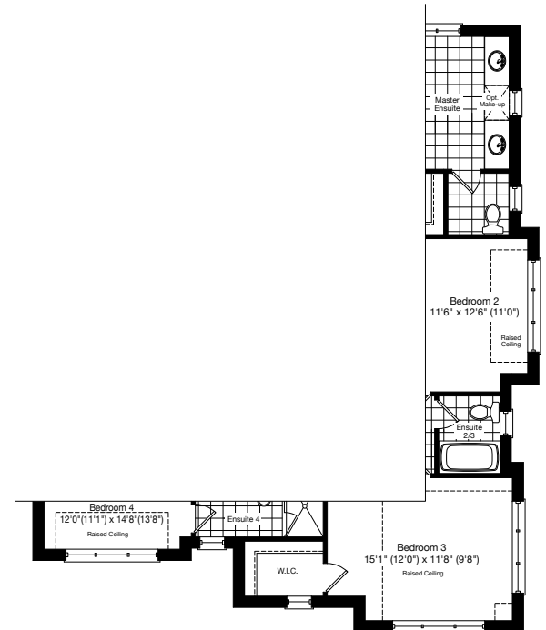
PARTIAL SECOND FLOOR ELEVATION B
